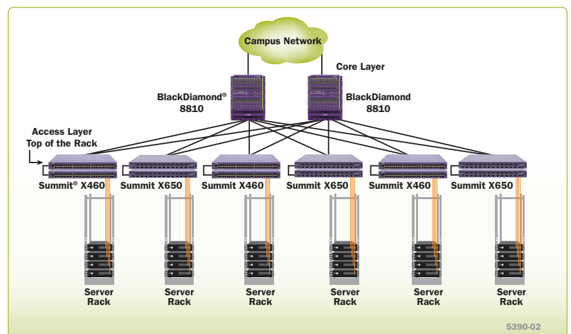
Figure 9: Top-of-Rack Architecture
