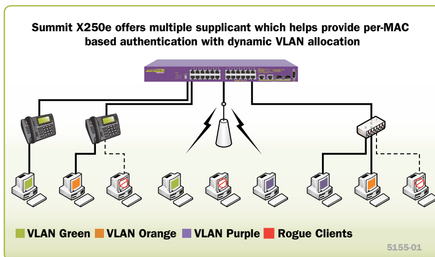
Figure 4: Multiple Supplicant Support
